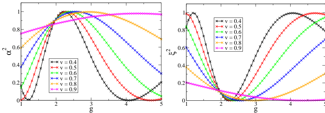
Figure 8: The Bogoliubov coefficients of the incoming K mode unto the outgoing K mode, |\alpha|^2 , (left) and B mode, |\xi|^2 , (right).
