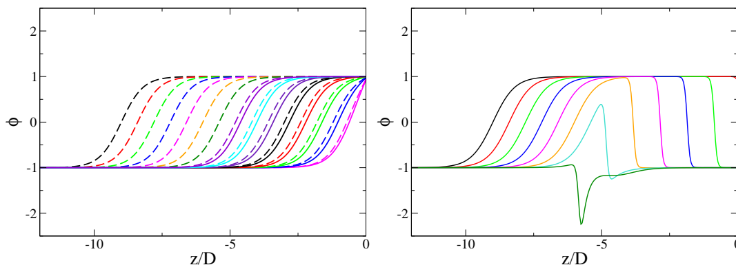
Figure 2: The incoming kink profiles before and after the collision with a -BC boundary (left). The curves are equally spaced in time, dashed before the collision, full after. The kink enters the boundary and comes back out unscathed. In contrast, the +BC boundary (right) decays straight away and emits an antikink which prevents the incoming kink from reaching the boundary.
