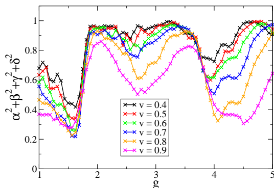
Figure 5: Left: The velocity and coupling dependence of the Bogoliubov coefficients of the K mode with the outgoing kink KE mode. Right: The same for the overlap on the antikink AE mode.
